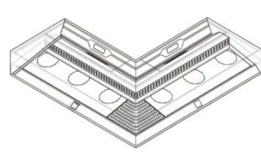
拐角油烟净化一体机 CORNER FUME PURIFICATION MACHINE
